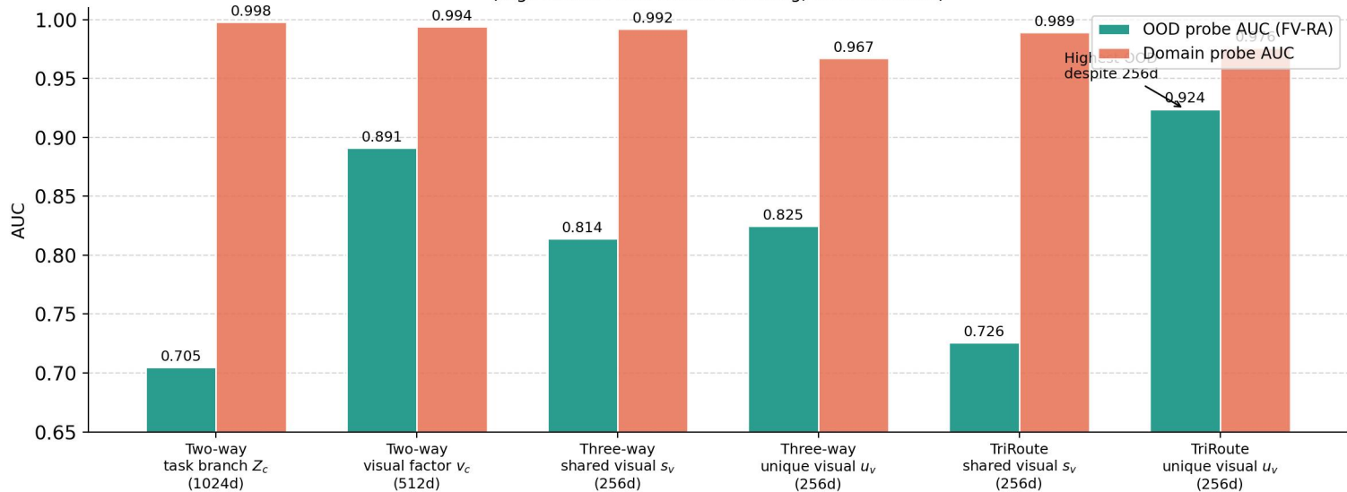
Subspace Probe: OOD vs Domain AUC (High domain AUC confirms routing, not invariance)
