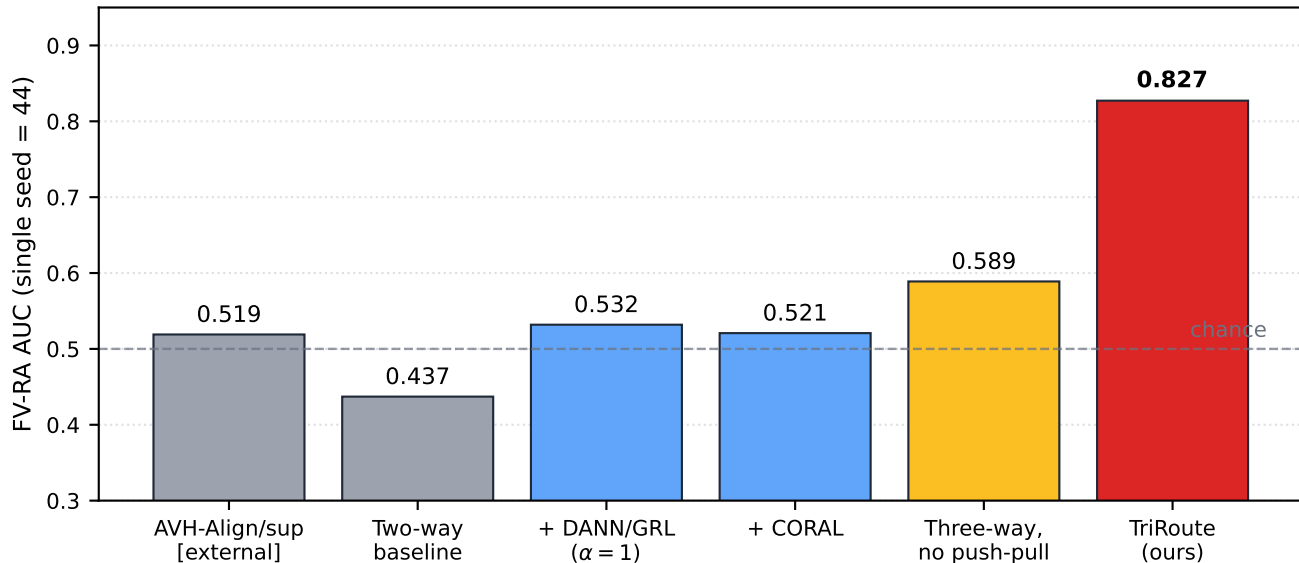
Cross-domain FV-RA AUC on FakeAVCeleb (AV1M \rightarrow FAVC, N = 3,158 , seed 44)
