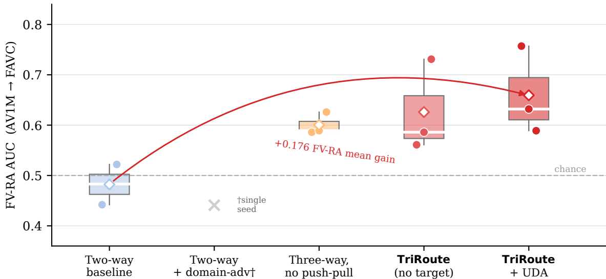
Per-seed FV-RA AUC across model variants ( \blacklozenge = mean, dots = individual seeds)
