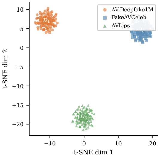
Domain factor H^d (colored by dataset)
