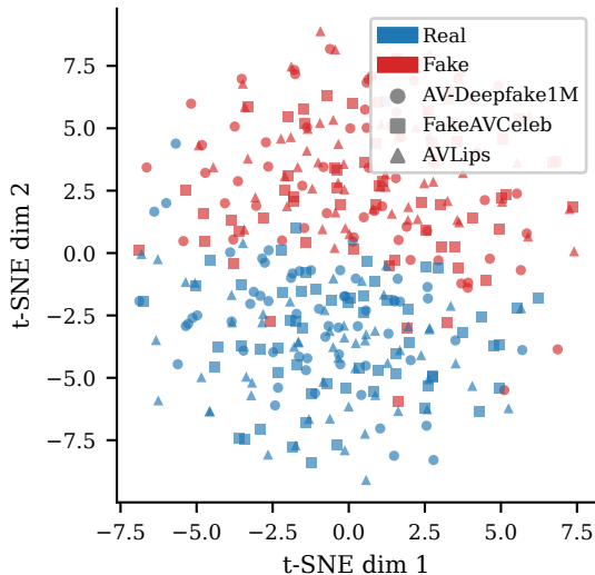
Manipulation factor H^m (colored by real/fake)
