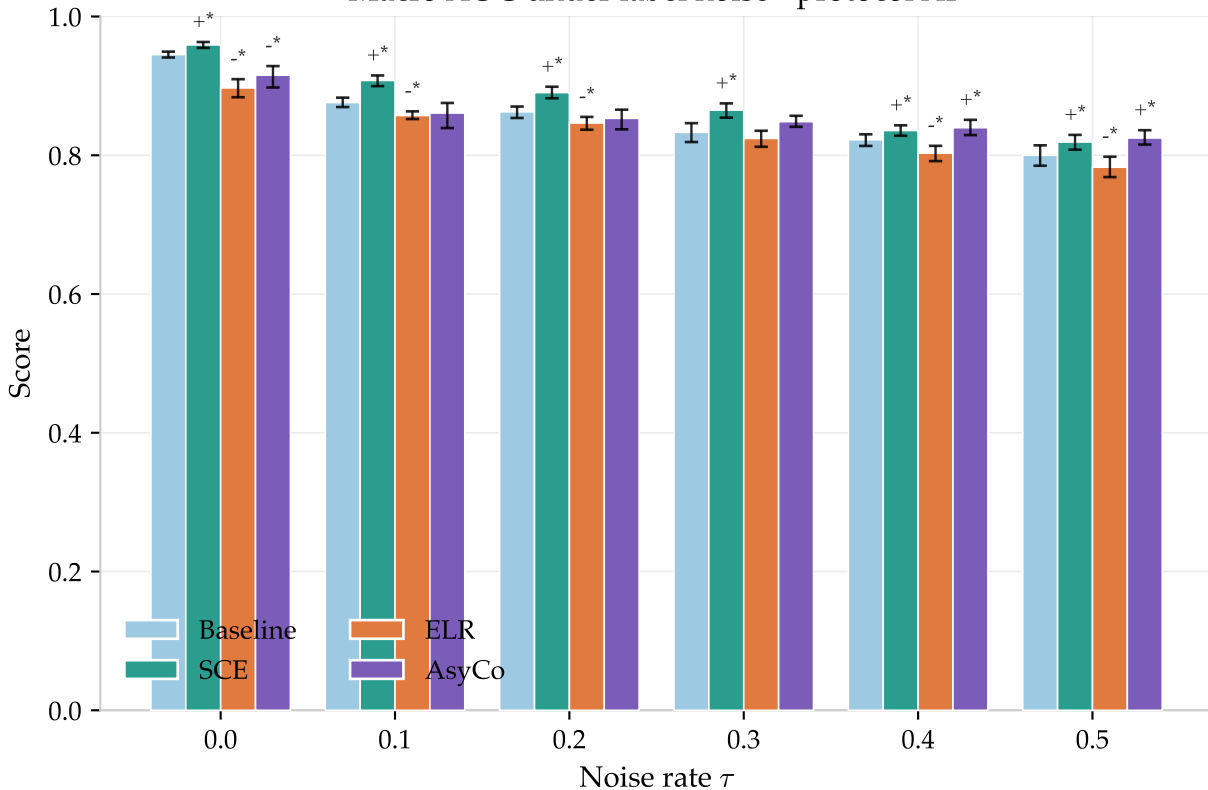
Macro AUC under label noise - protocol AP
