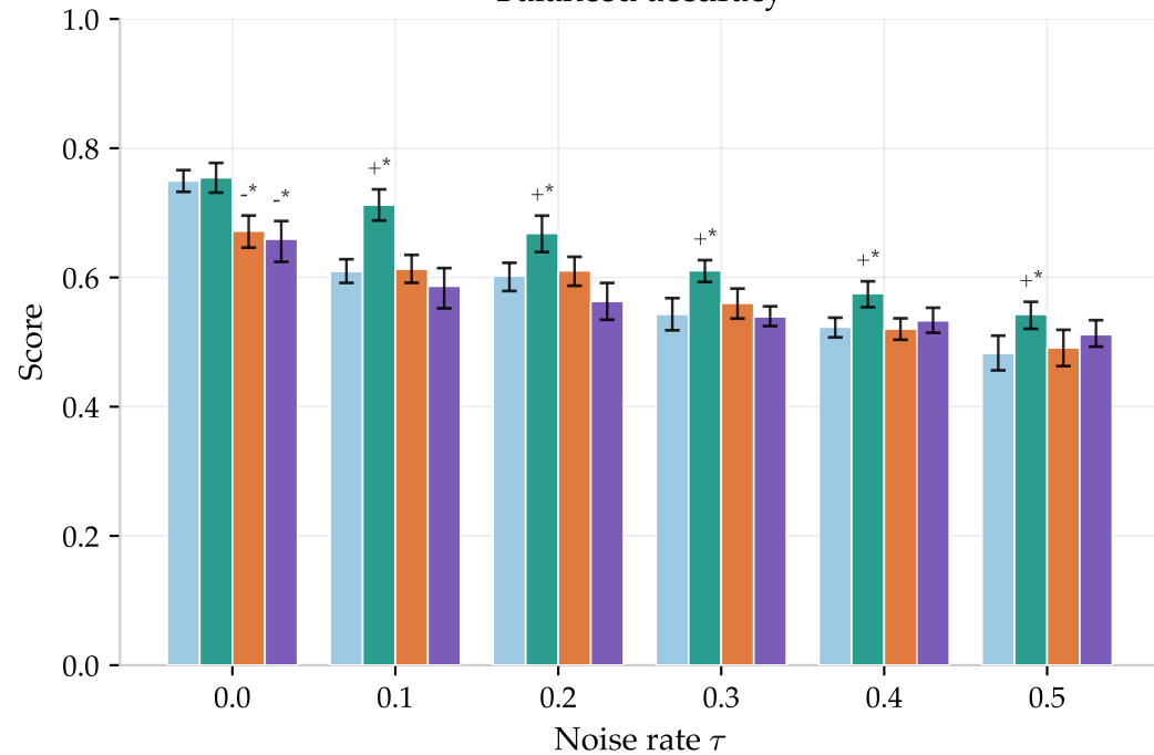
Balanced accuracy
