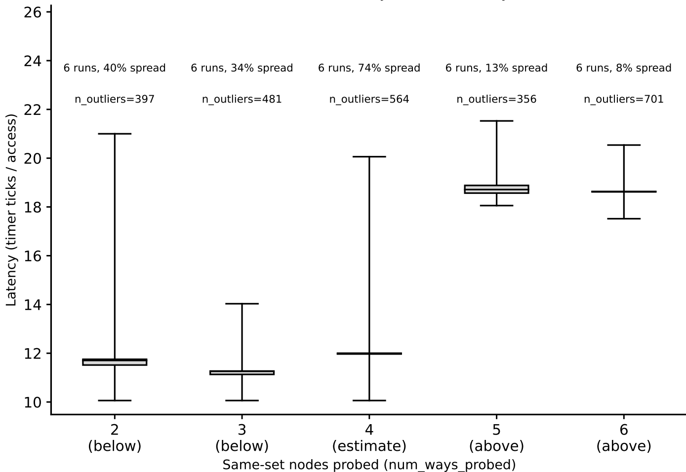
sunbird: associativity box plots, L2_256KiB_candidate, random pattern (whiskers = p5/p95) (Phase I timing-only; order-sensitive across seeds, see README) detected associativity estimate: 4-way
