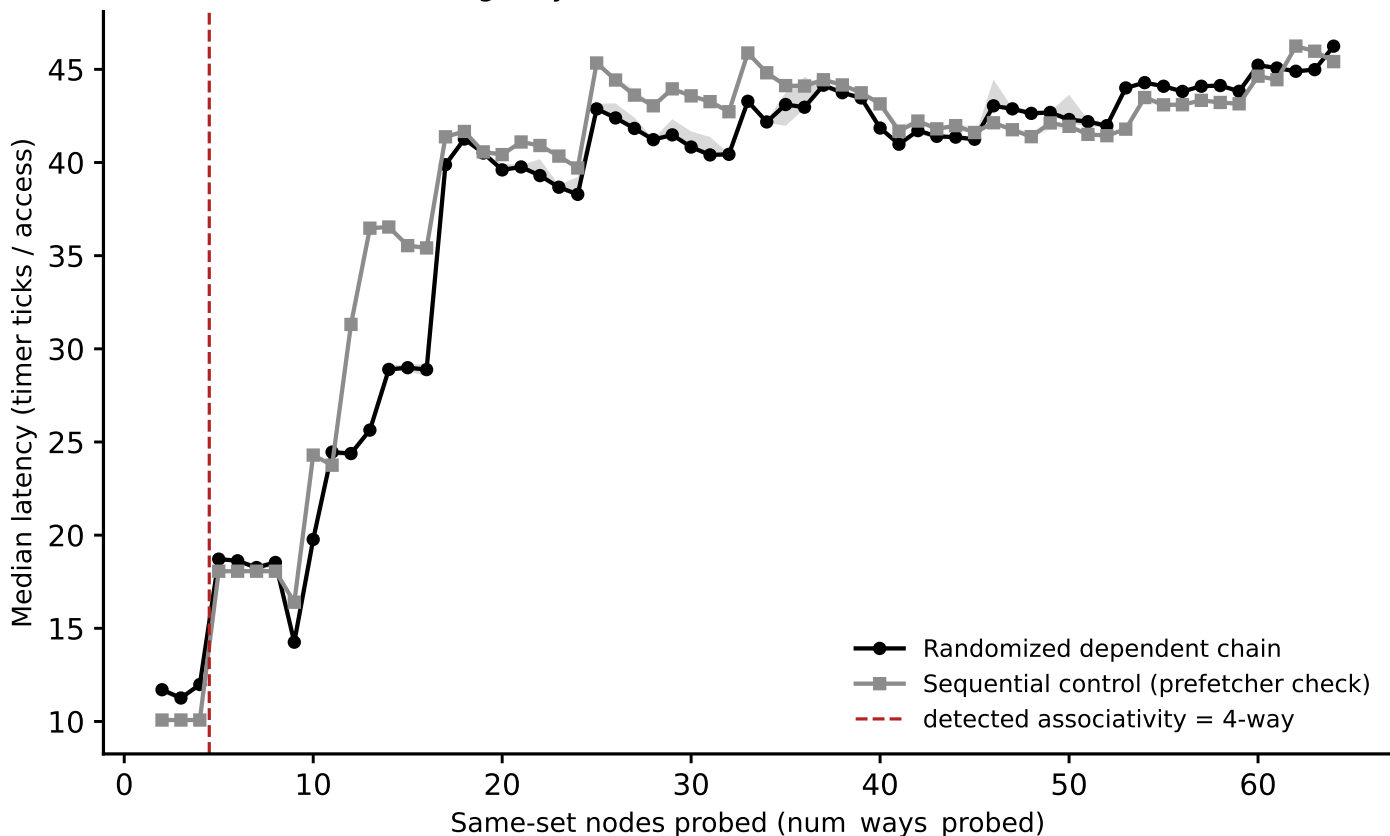
sunbird: associativity sweep, L2_256KiB_candidate (stride=256 KiB) (Phase I timing-only; order-sensitive across seeds, see README)
