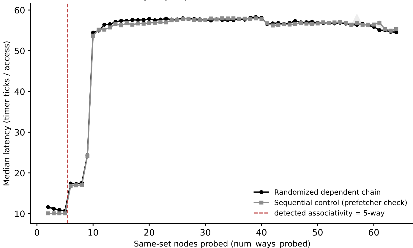
sunbird: associativity sweep, LLC_32MiB (stride=32 MiB) (Phase I timing-only; reproducible across 3 seeds, see README)
