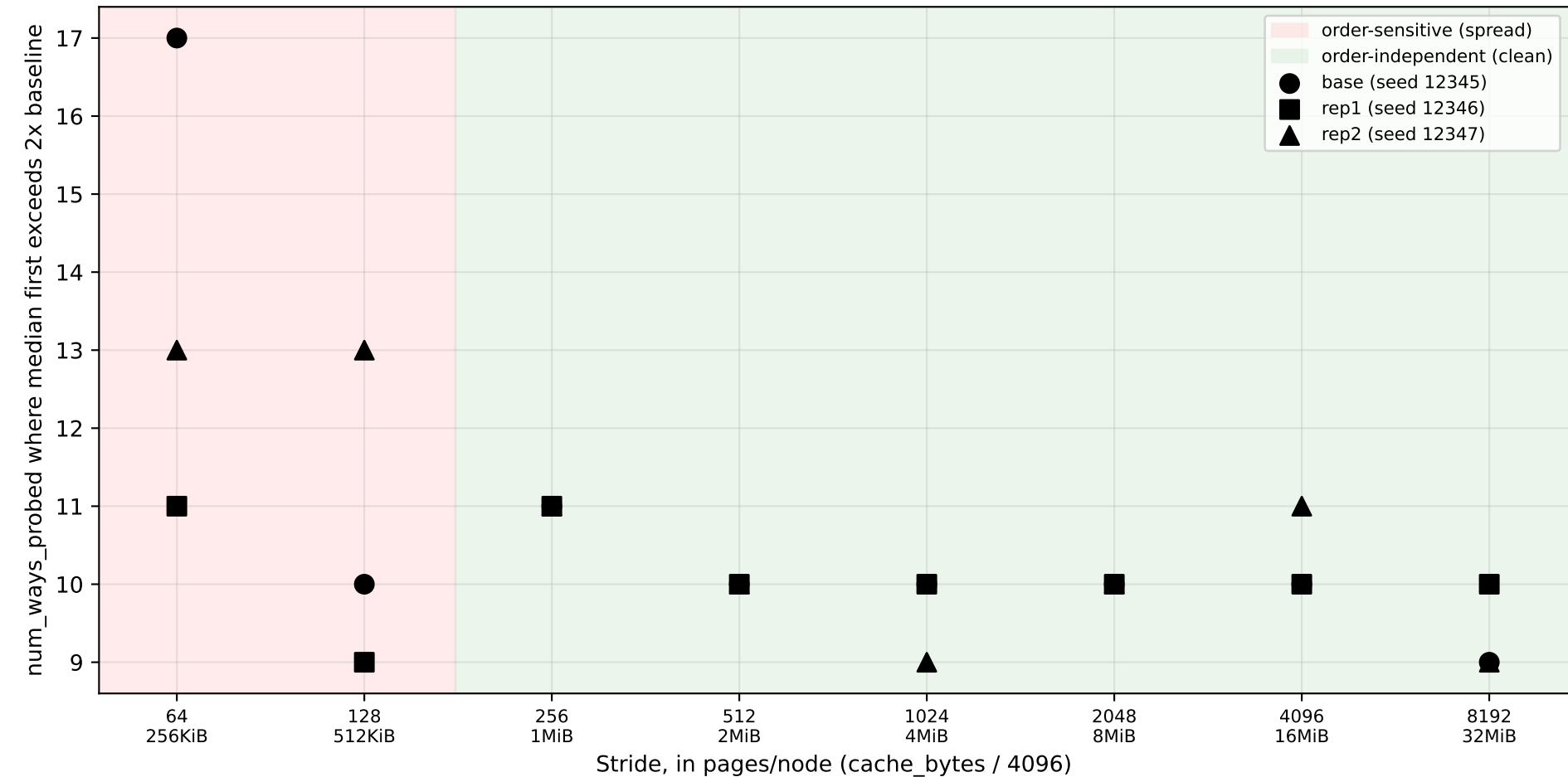
sunbird: associativity-knee order-sensitivity vs. stride (Phase I timing-only, 3 seeds per candidate)
