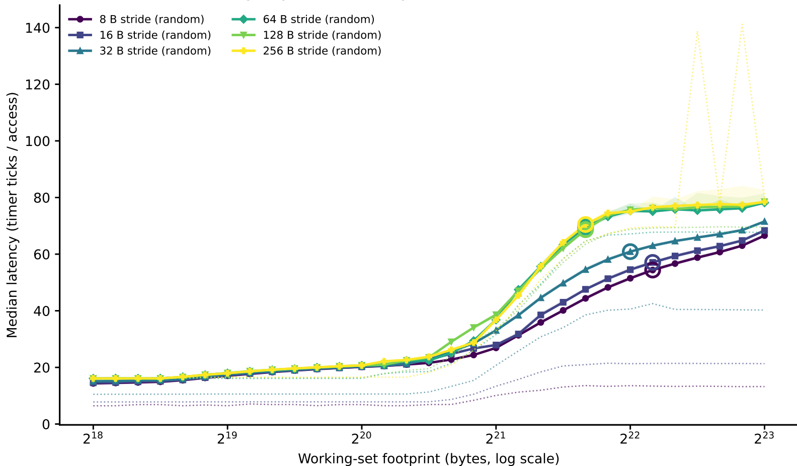
artemisia: line-size family of curves (dependent pointer chase) (Phase I timing-only, level boundary=2097152B window=[262144,8388608])
