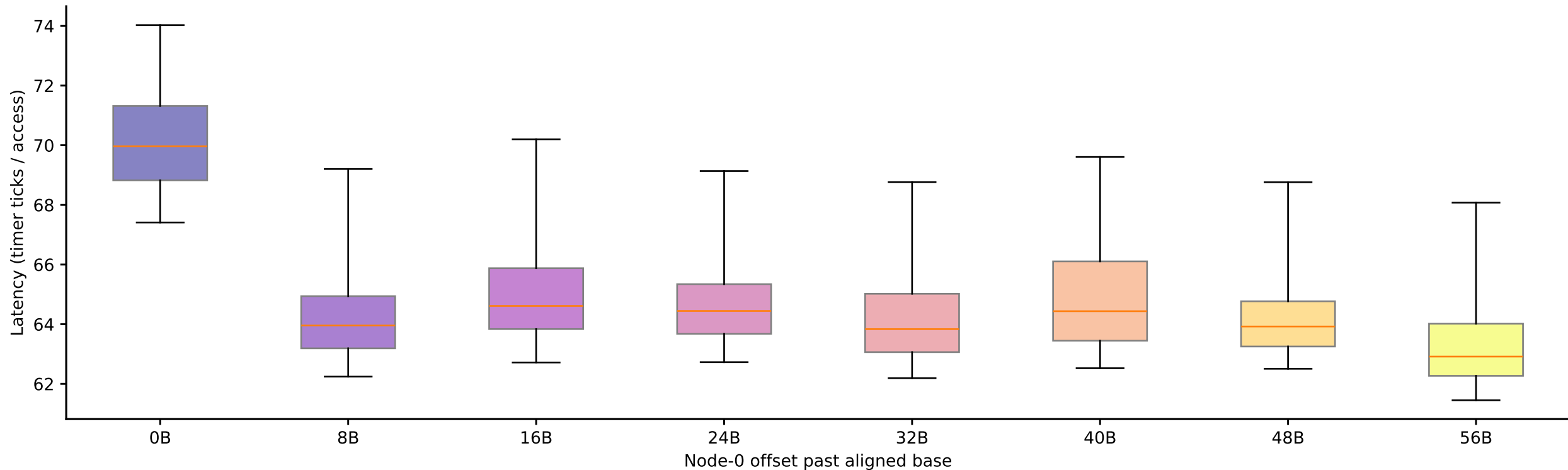
artemisia: candidate stride 64 B at footprint 2.82837 MiB, by offset (Phase I timing-only, level boundary=2097152B, step-4 alignment refinement)
