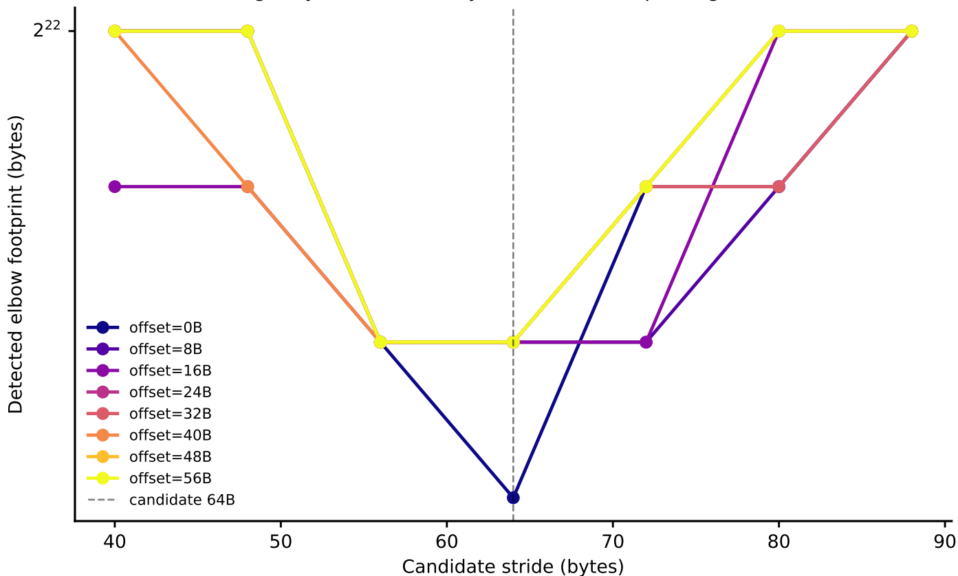
artemisia: line-size elbow vs. stride, by node-0 offset (Phase I timing-only, level boundary=2097152B, step-4 alignment refinement)
