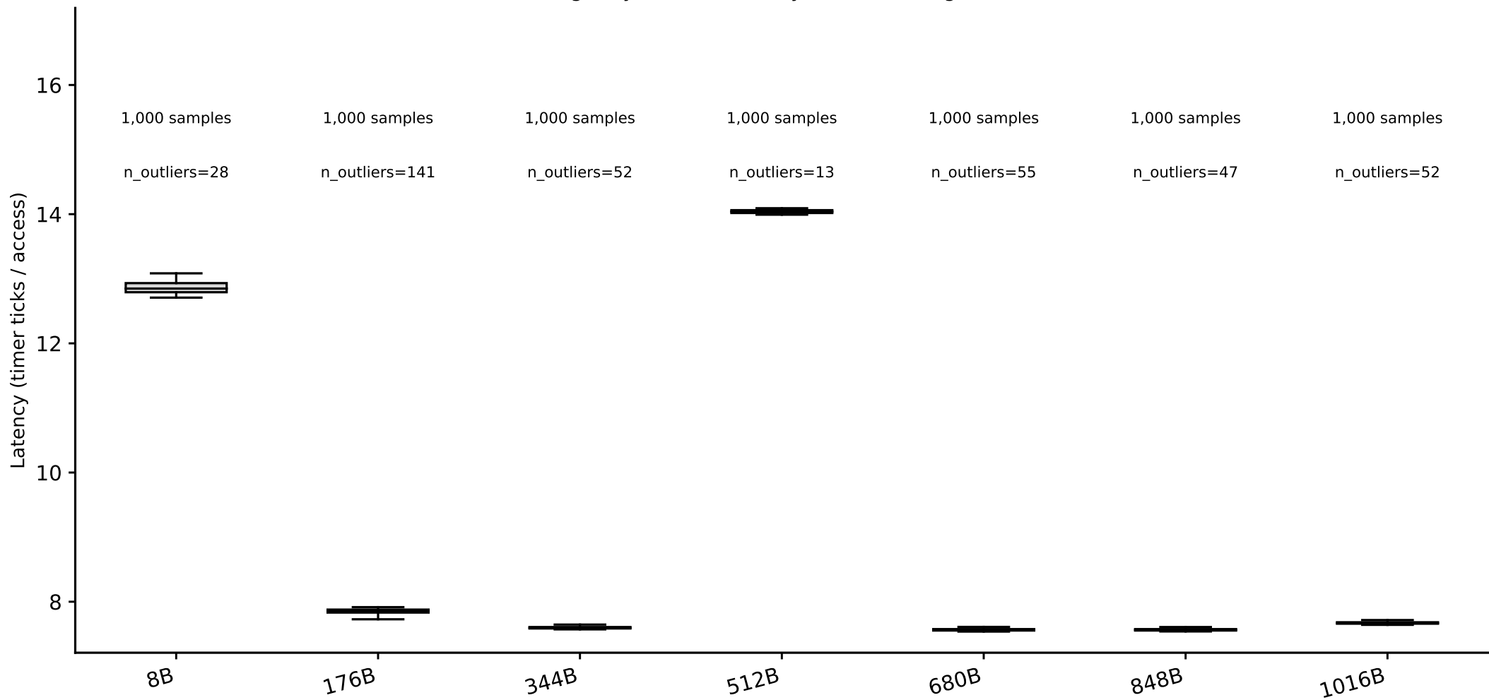
charnwood: line-size box plots, random pattern (whiskers = p5/p95) (Phase I timing-only, level boundary=32768B, single-curve method)
