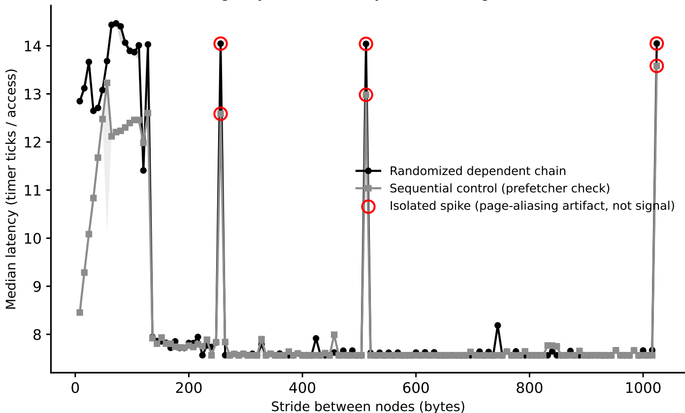
charnwood: line-size sweep (dependent pointer chase), footprint=64 KiB (Phase I timing-only, level boundary=32768B, single-curve method)
