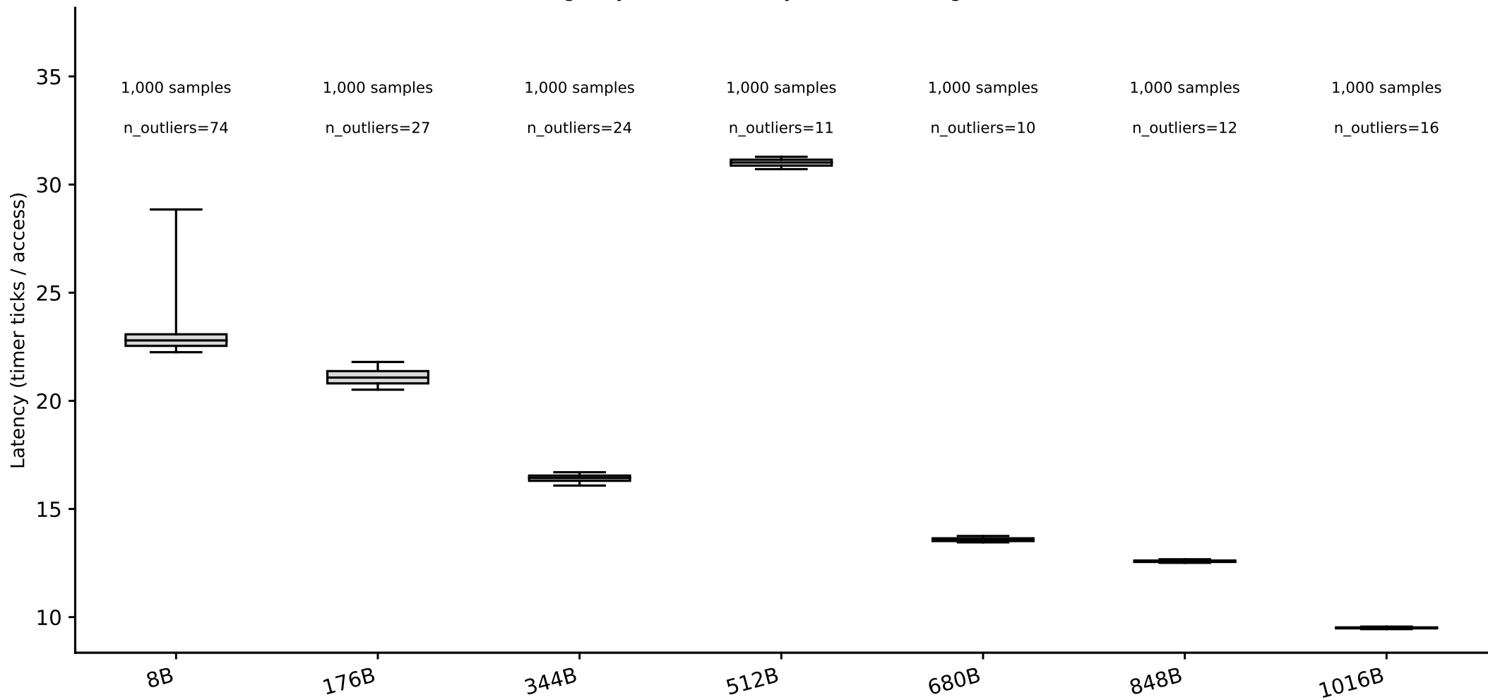
crux: line-size box plots, random pattern (whiskers = p5/p95) (Phase I timing-only, level boundary=262144B, single-curve method)
