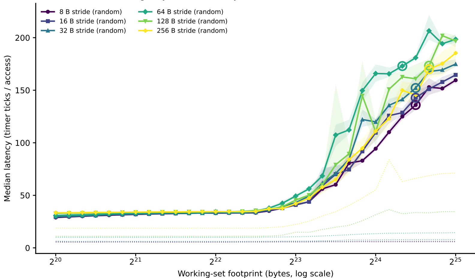
crux: line-size family of curves (dependent pointer chase) (Phase I timing-only, level boundary=8388608B window=[1048576,33554432])
