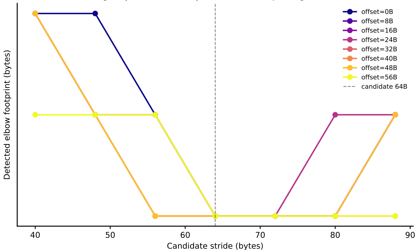
crux: line-size elbow vs. stride, by node-0 offset (Phase I timing-only, level boundary=8388608B, step-4 alignment refinement)
