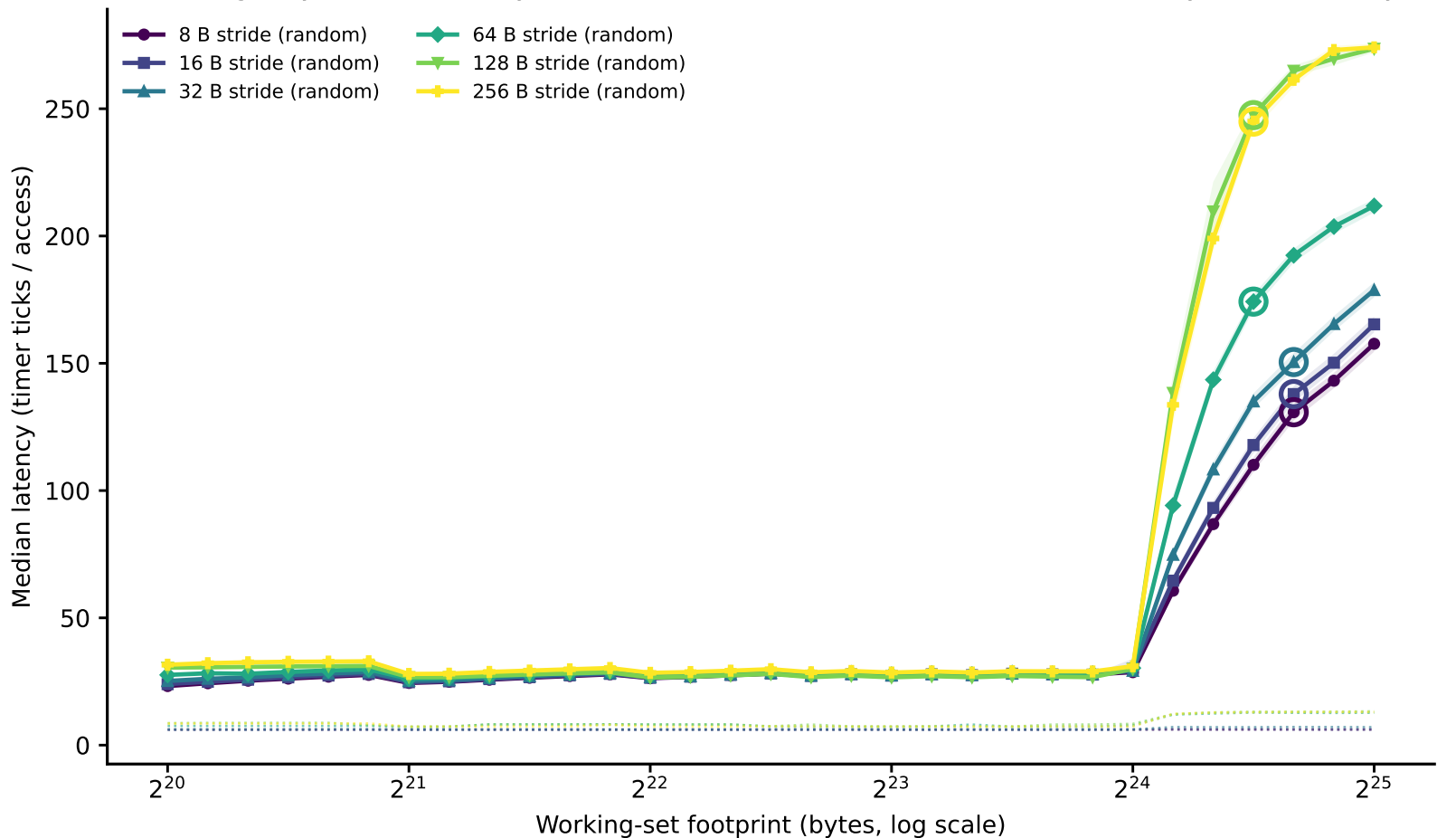
skylark: line-size family of curves (dependent pointer chase) (Phase I timing-only, level boundary=8388608B window=[1048576,33554432], family-of-curves-only reru
