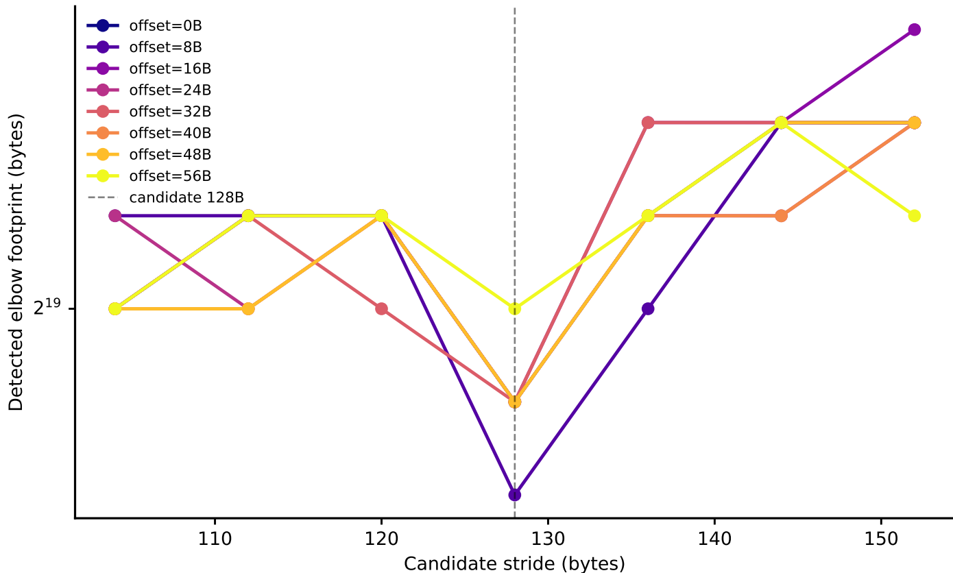
upgrade: line-size elbow vs. stride, by node-0 offset (Phase I timing-only, level boundary=262144B, step-4 alignment refinement)
