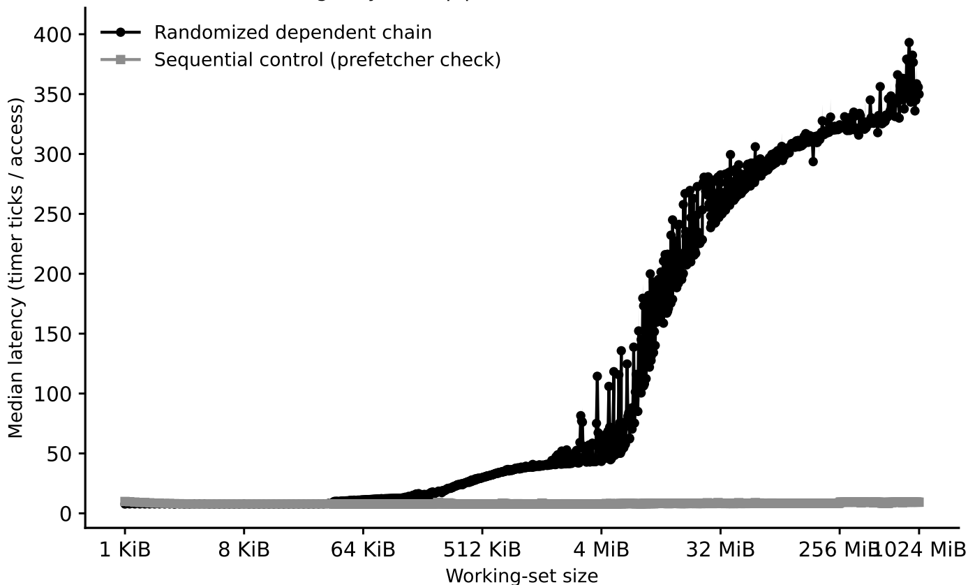
charnwood: capacity sweep (dependent pointer chase) (Phase I timing-only, auto pipeline + manual tail extension to 1GiB)
