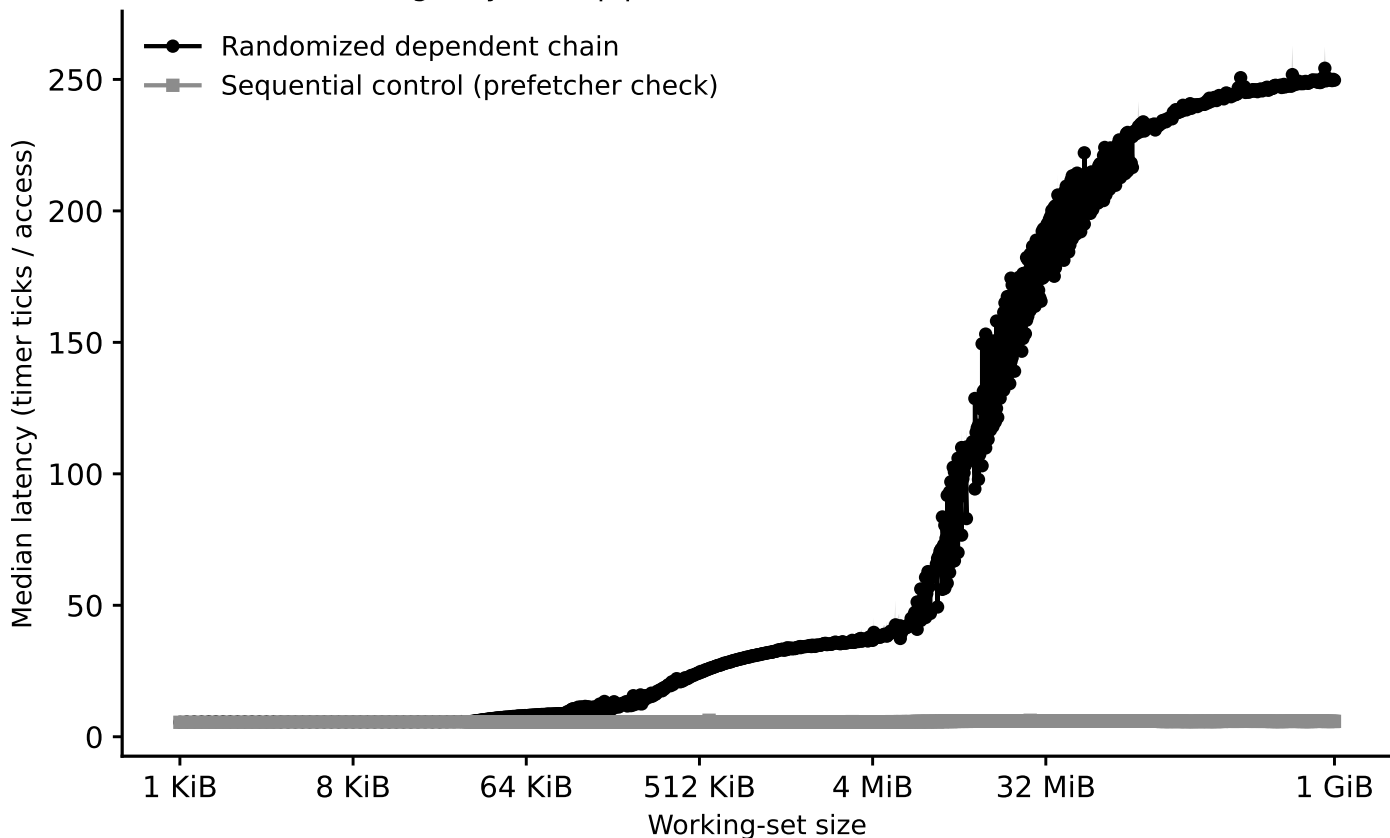
crux: capacity sweep (dependent pointer chase) (Phase I timing-only, auto pipeline + manual tail-extension2 256MiB-1GiB)
