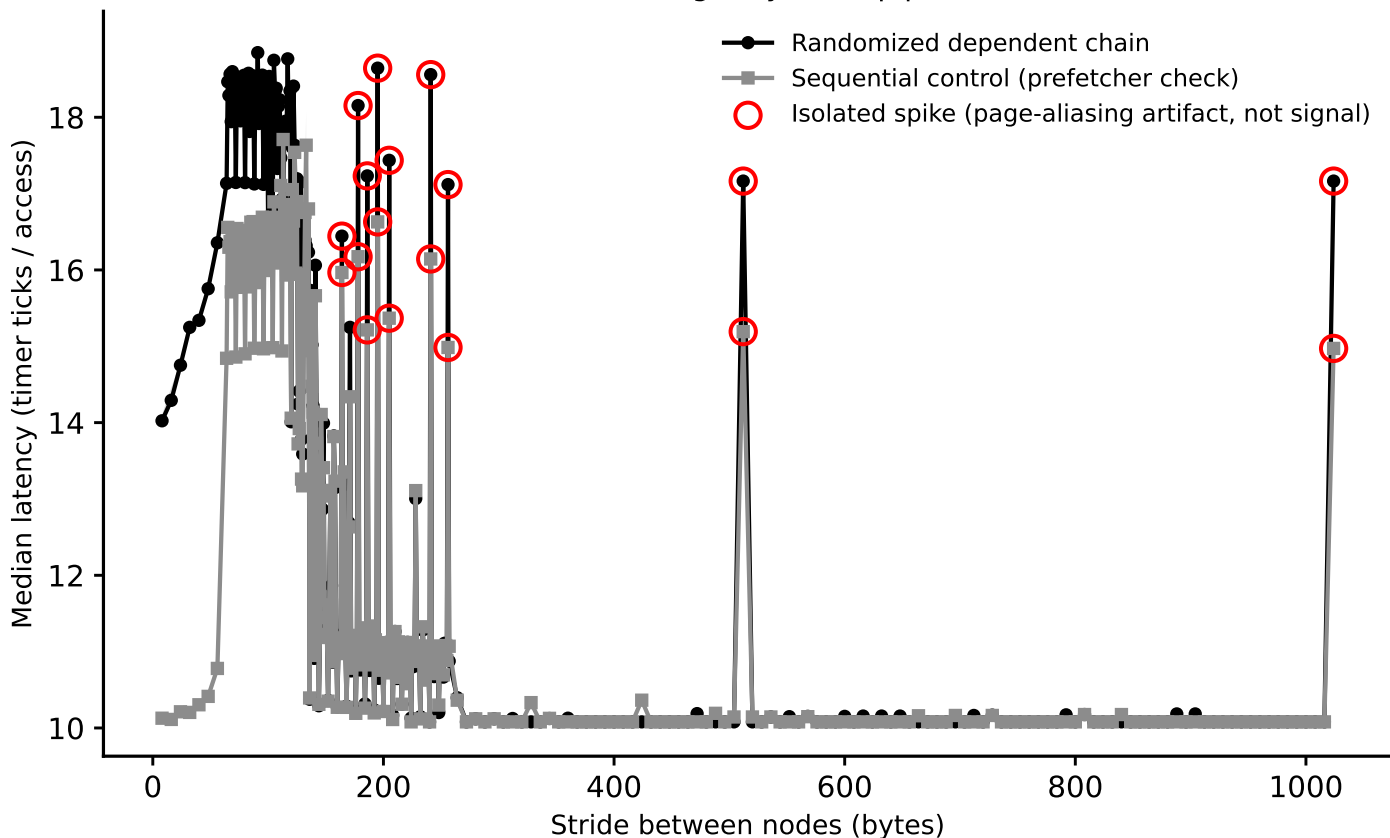
sunbird: line-size sweep (dependent pointer chase), footprint=64 KiB (Phase I timing-only, auto pipeline)
