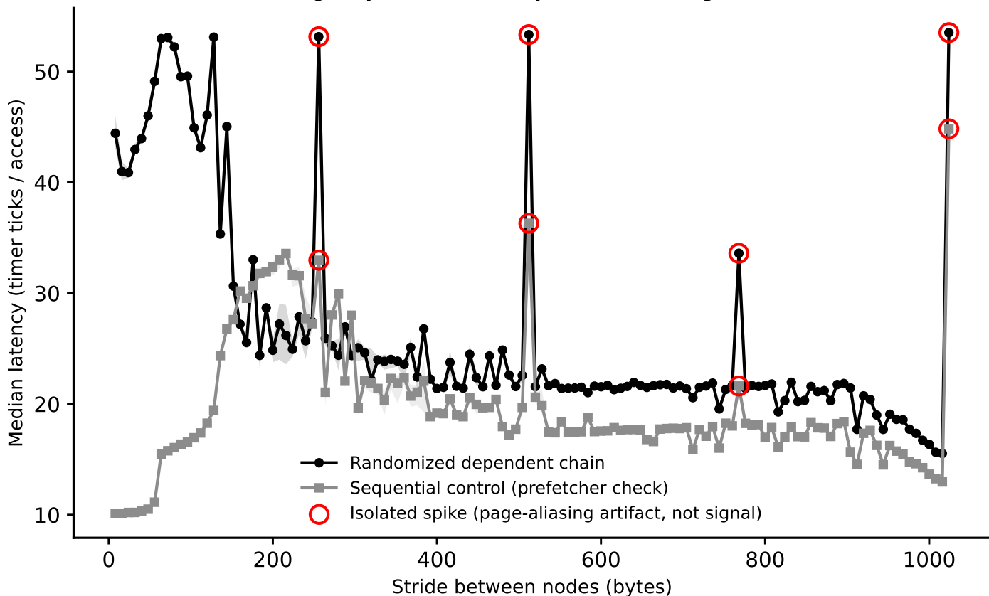
sunbird: line-size sweep (dependent pointer chase), footprint=512 KiB (Phase I timing-only, level boundary=262144B, single-curve method)
