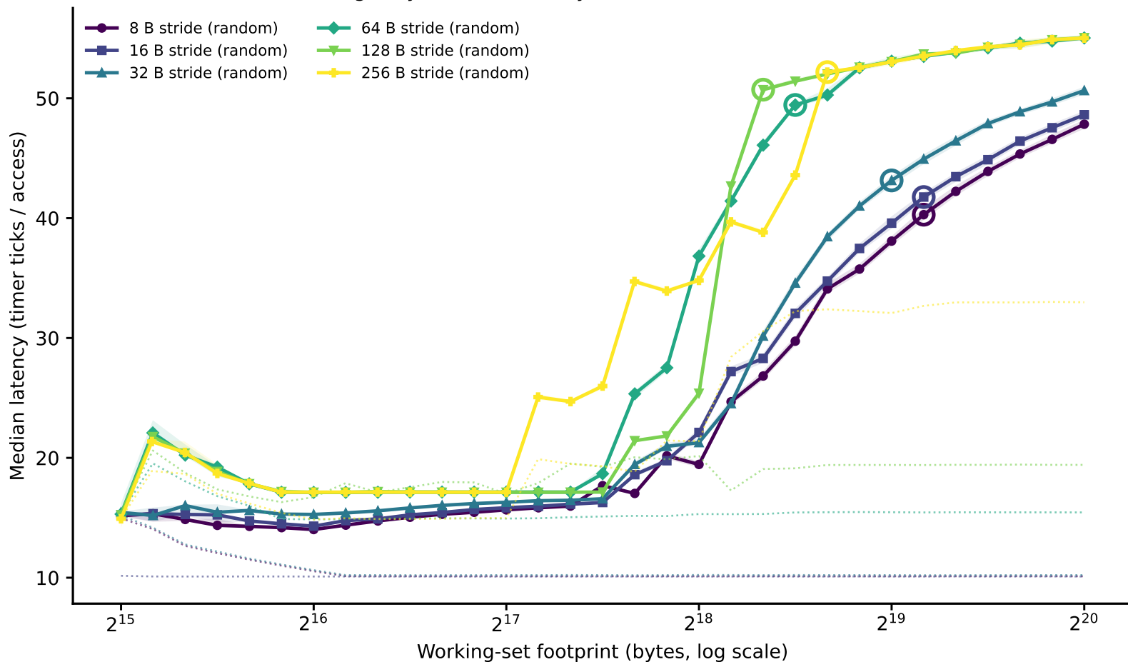
sunbird: line-size family of curves (dependent pointer chase) (Phase I timing-only, level boundary=262144B window=[32768,1048576])
