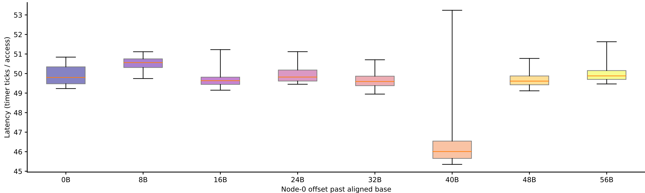
sunbird: candidate stride 64 B at footprint 406.375 KiB, by offset (Phase I timing-only, level boundary=262144B, step-4 alignment refinement)
