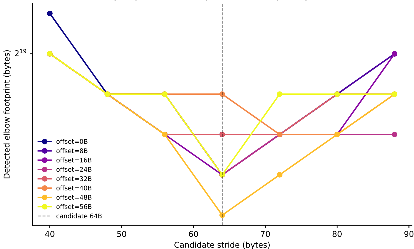
sunbird: line-size elbow vs. stride, by node-0 offset (Phase I timing-only, level boundary=262144B, step-4 alignment refinement)
