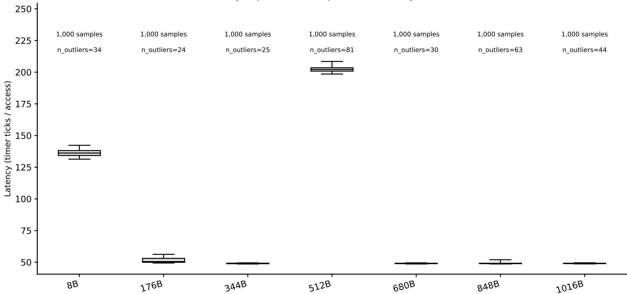
sunbird: line-size box plots, random pattern (whiskers = p5/p95) (Phase I timing-only, level boundary=31457280B, single-curve method)
