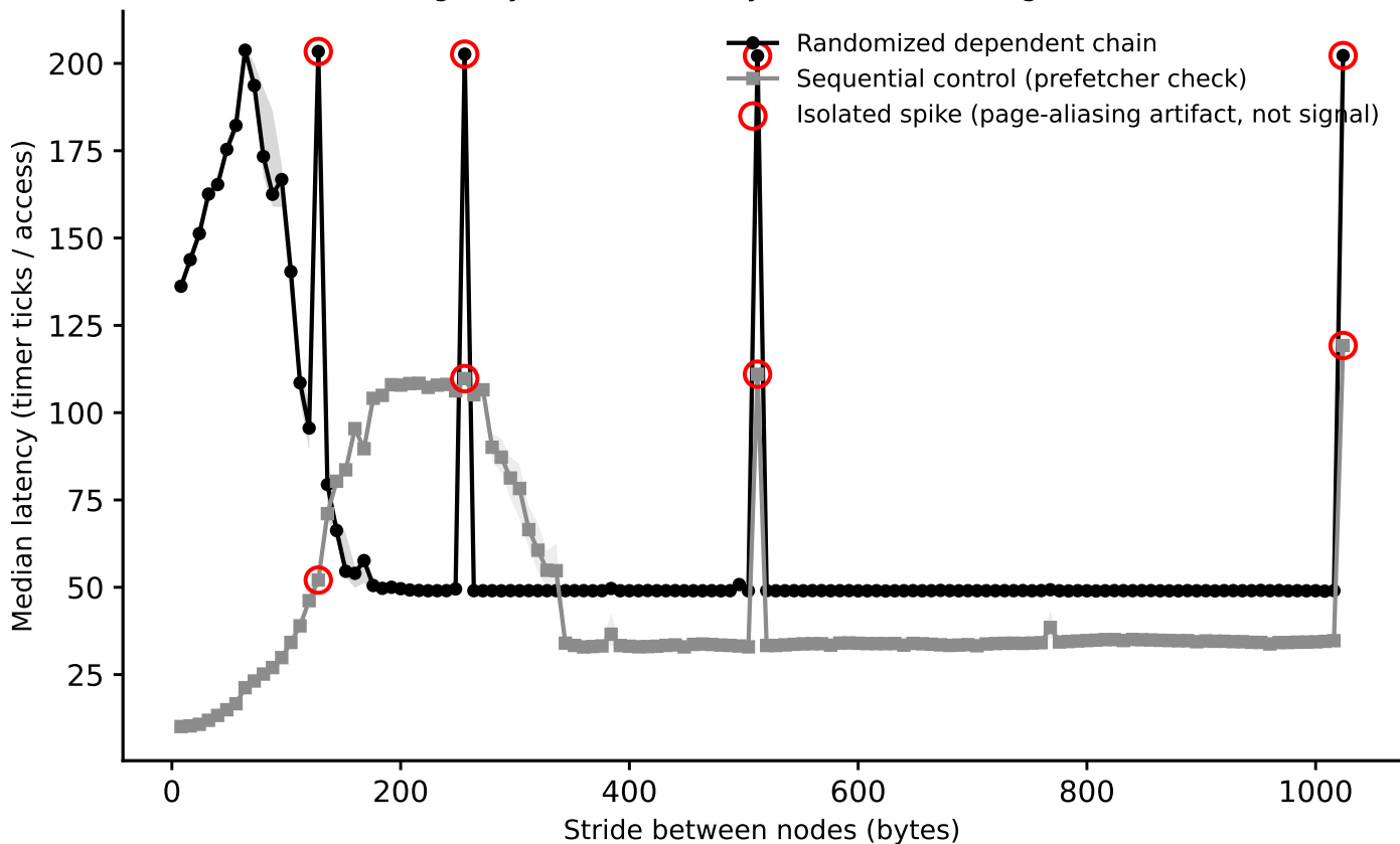
sunbird: line-size sweep (dependent pointer chase), footprint=60 MiB (Phase I timing-only, level boundary=31457280B, single-curve method)
