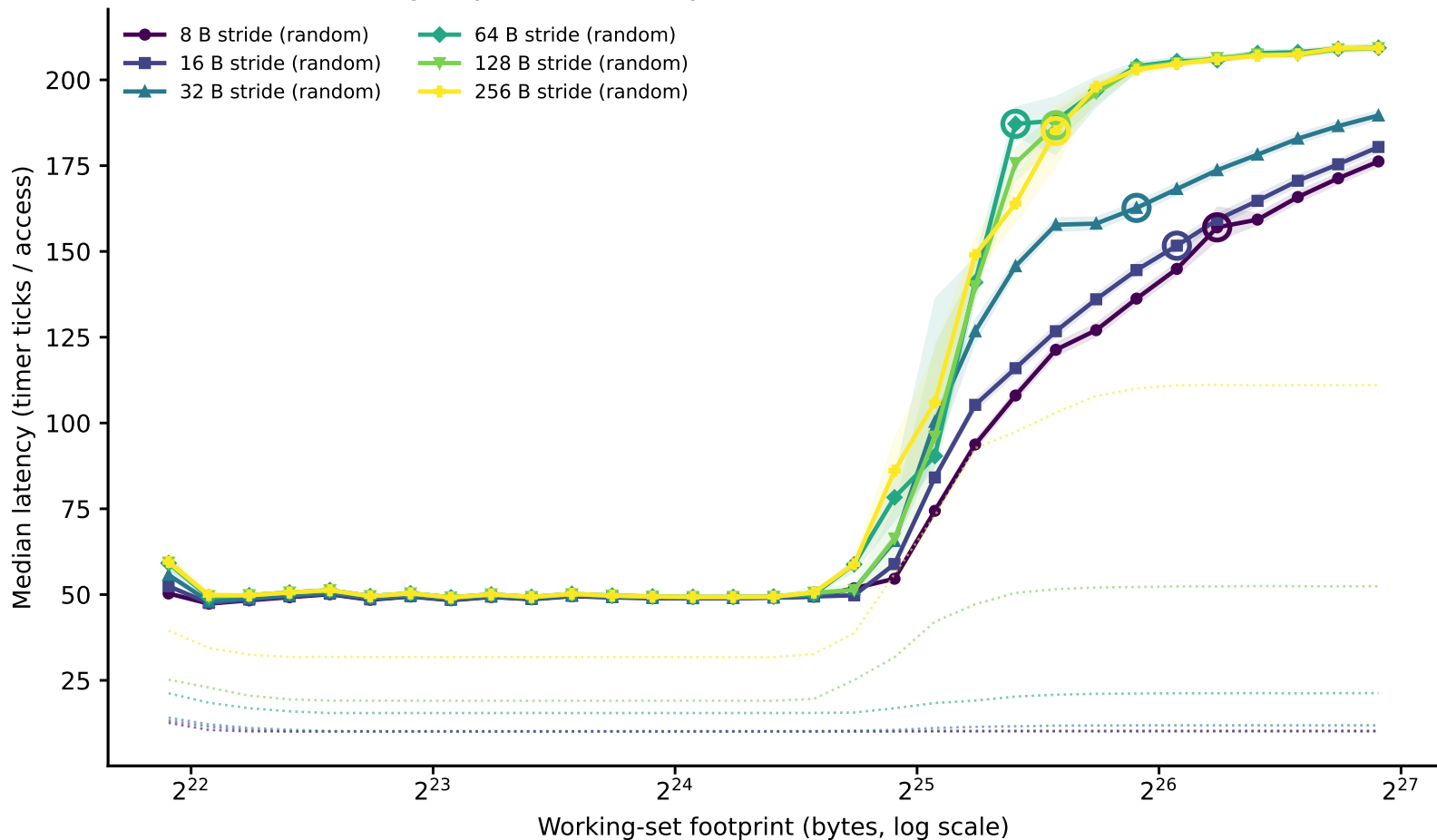
sunbird: line-size family of curves (dependent pointer chase) (Phase I timing-only, level boundary=31457280B window=[3932160,125829120])
