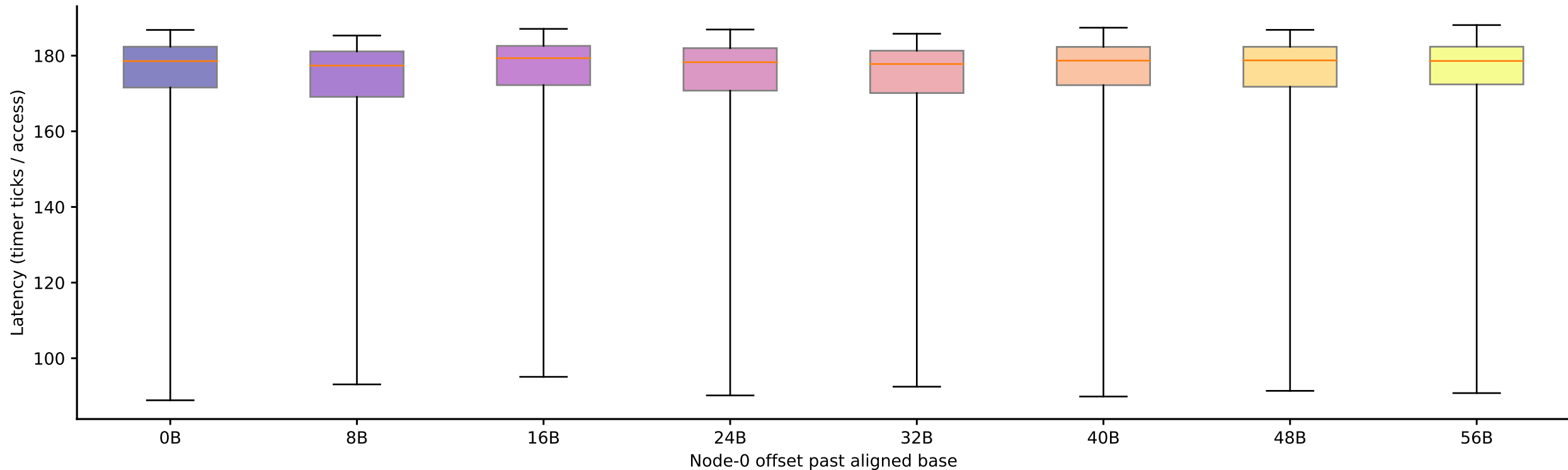
sunbird: candidate stride 64 B at footprint 42.4264 MiB, by offset (Phase I timing-only, level boundary=31457280B, step-4 alignment refinement)
