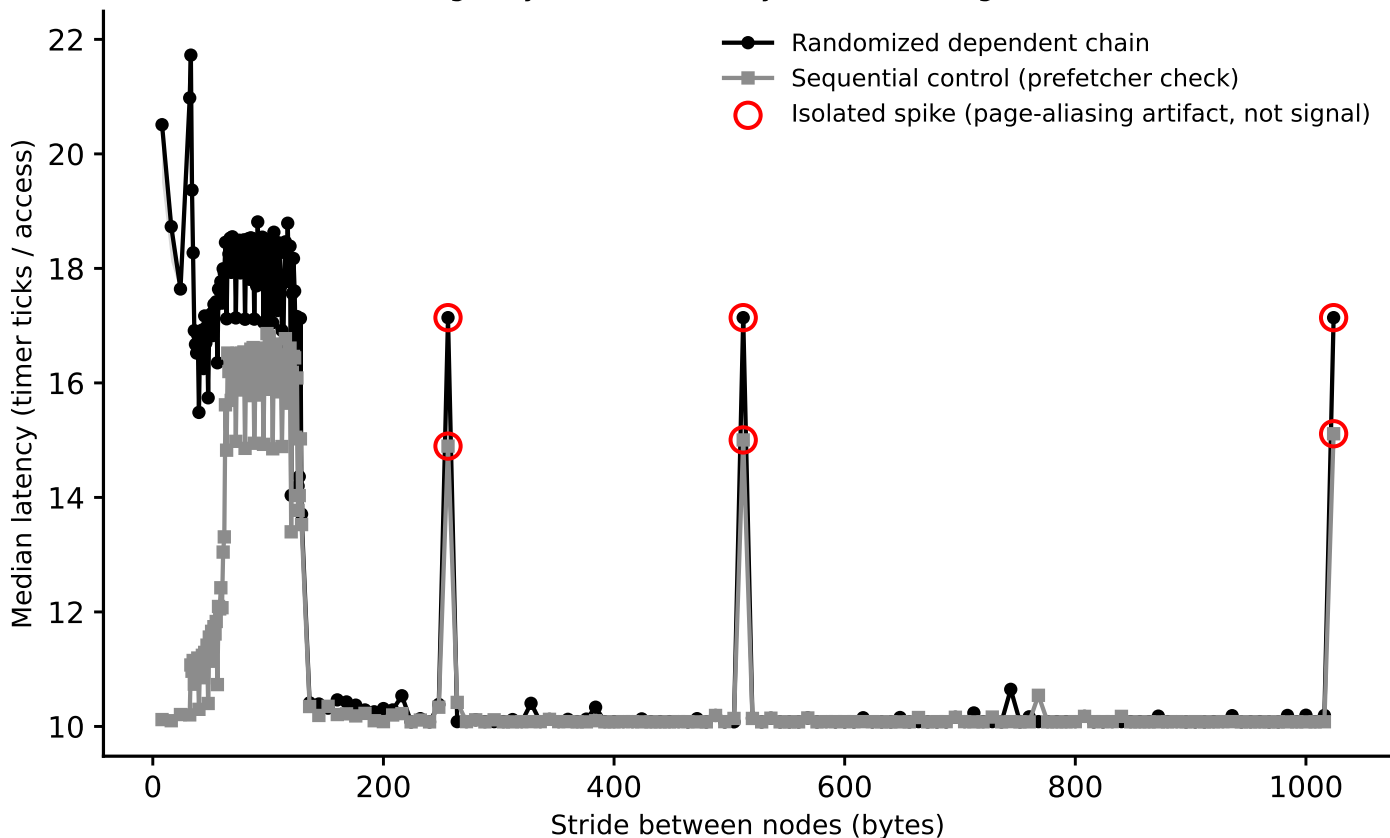
sunbird: line-size sweep (dependent pointer chase), footprint=64 KiB (Phase I timing-only, level boundary=32768B, single-curve method)
