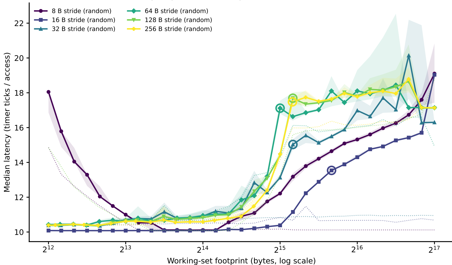
sunbird: line-size family of curves (dependent pointer chase) (Phase I timing-only, level boundary=32768B window=[4096,131072])
