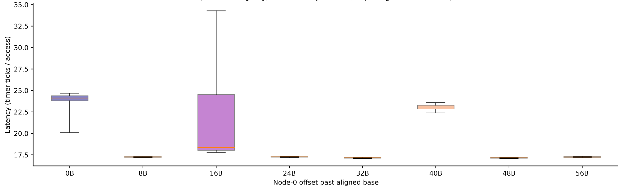
sunbird: candidate stride 64 B at footprint 114 KiB, by offset (Phase I timing-only, level boundary=32768B, step-4 alignment refinement)
