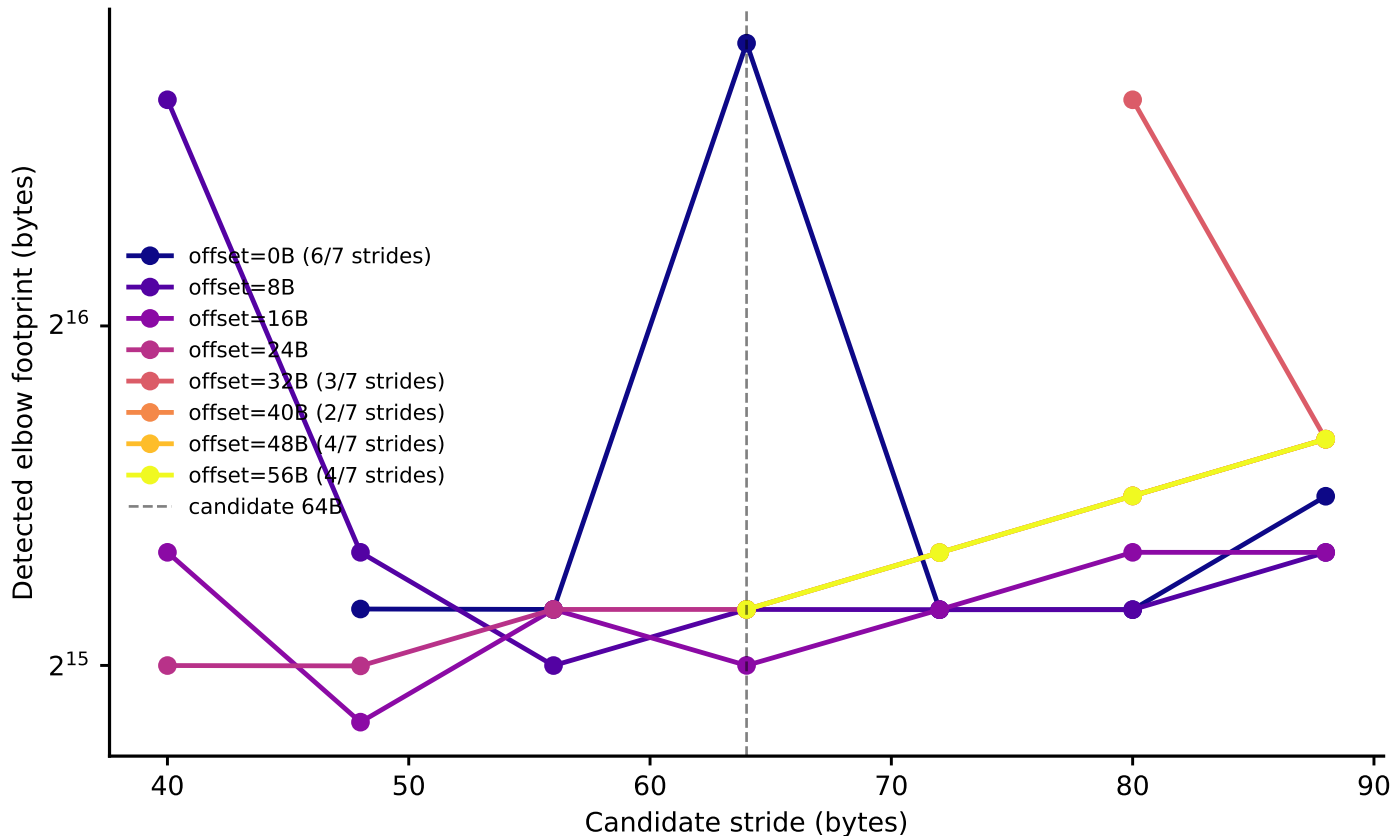
sunbird: line-size elbow vs. stride, by node-0 offset (Phase I timing-only, level boundary=32768B, step-4 alignment refinement)
