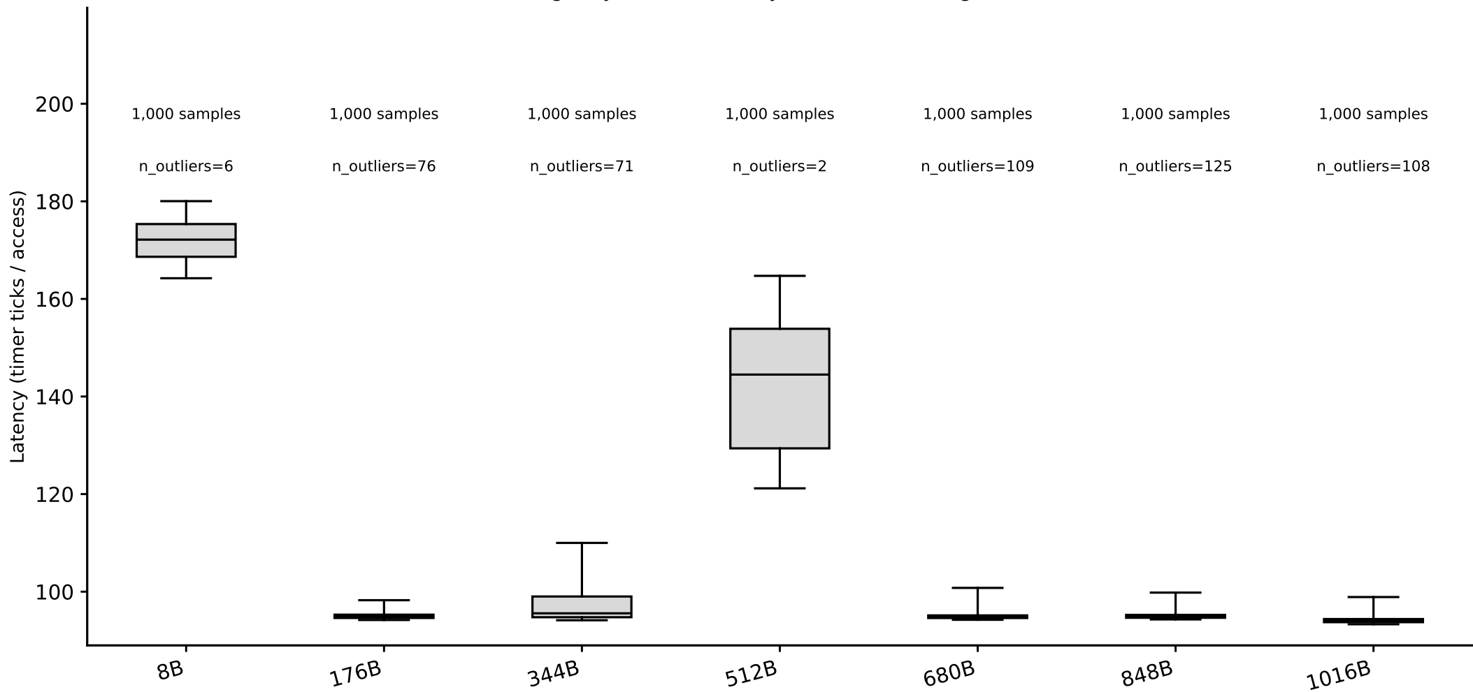
artemis: line-size box plots, random pattern (whiskers = p5/p95) (Phase I timing-only, level boundary=31457280B, single-curve method)
