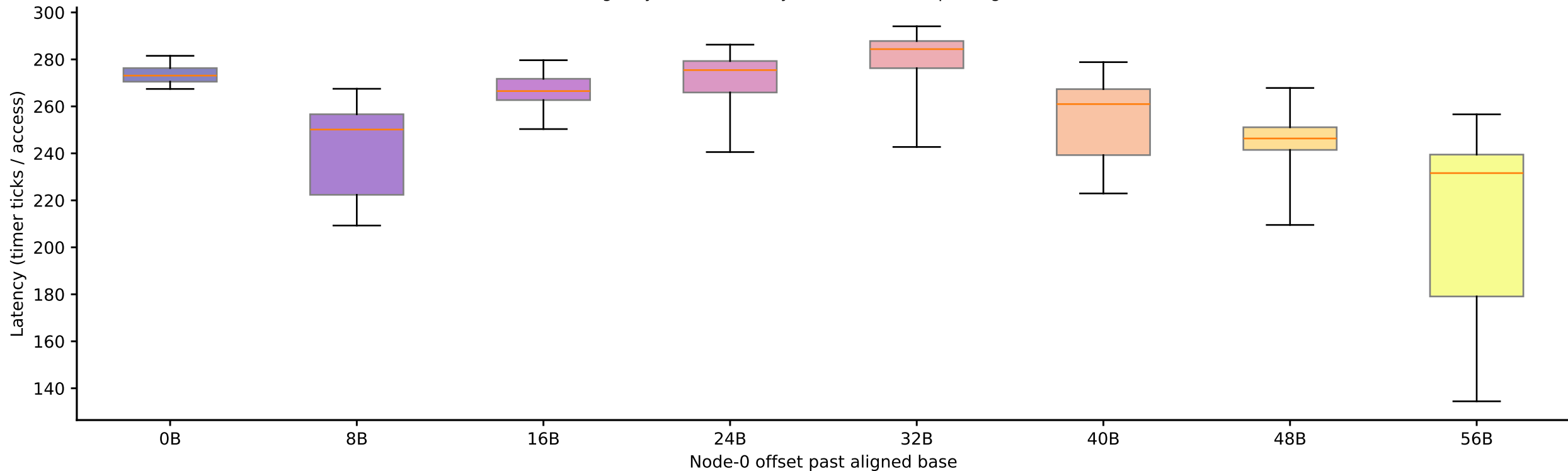
artemisia: candidate stride 64 B at footprint 75.5952 MiB, by offset (Phase I timing-only, level boundary=31457280B, step-4 alignment refinement)
