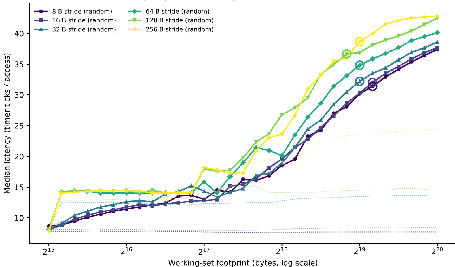
charnwood: line-size family of curves (dependent pointer chase) (Phase I timing-only, level boundary=262144B window=[32768,1048576])
