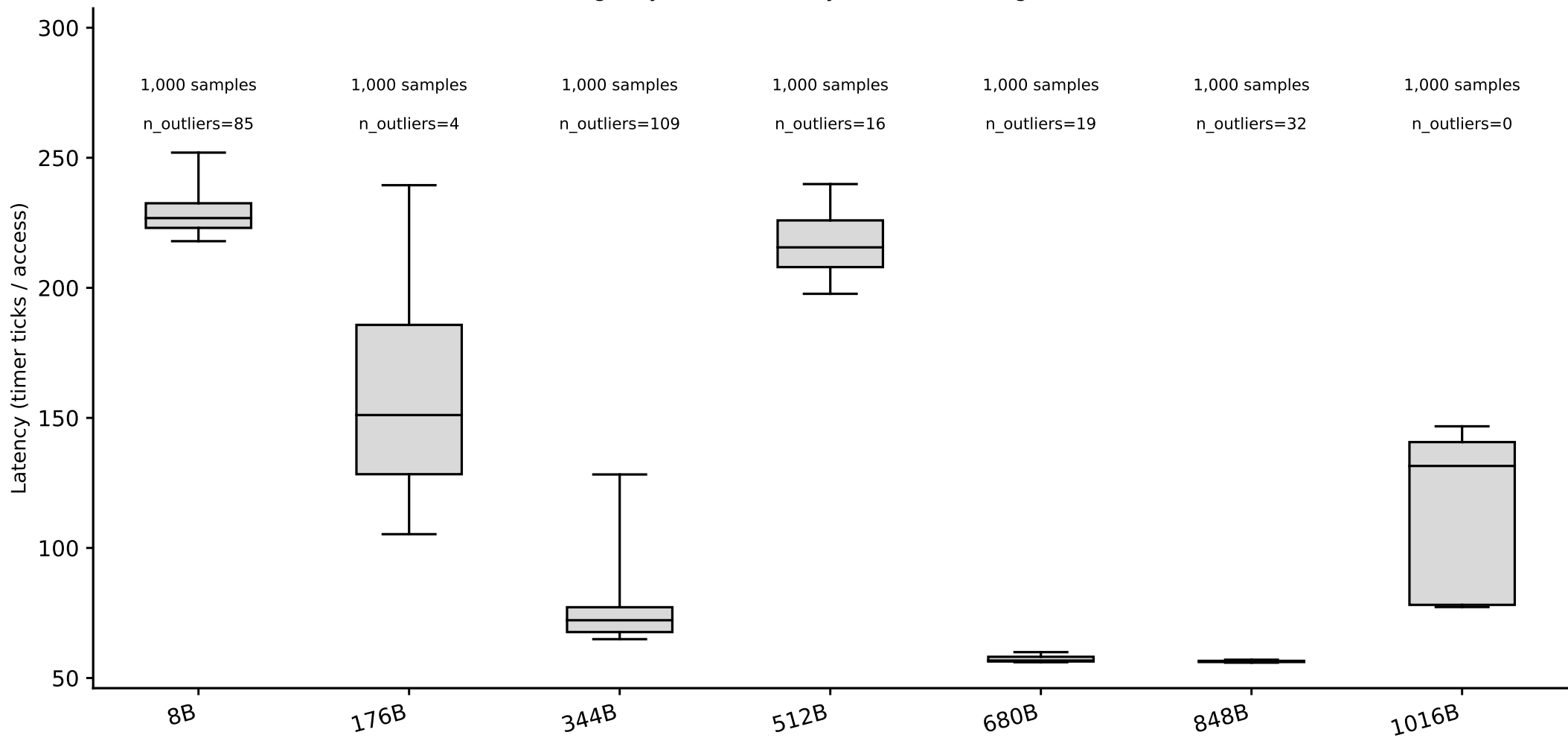
charnwood: line-size box plots, random pattern (whiskers = p5/p95) (Phase I timing-only, level boundary=8388608B, single-curve method)
