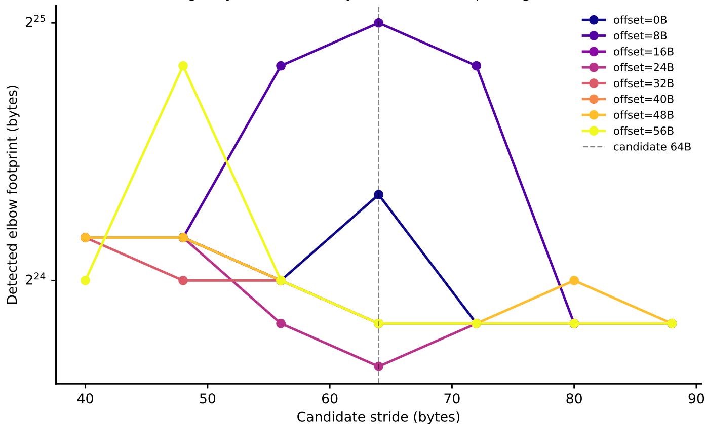
charnwood: line-size elbow vs. stride, by node-0 offset (Phase I timing-only, level boundary=8388608B, step-4 alignment refinement)
