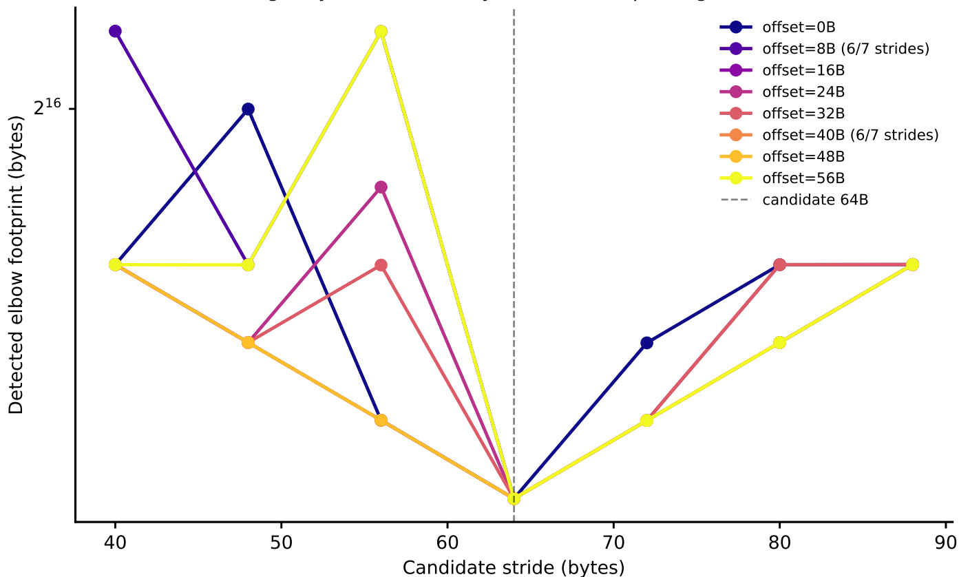
crux: line-size elbow vs. stride, by node-0 offset (Phase I timing-only, level boundary=32768B, step-4 alignment refinement)
