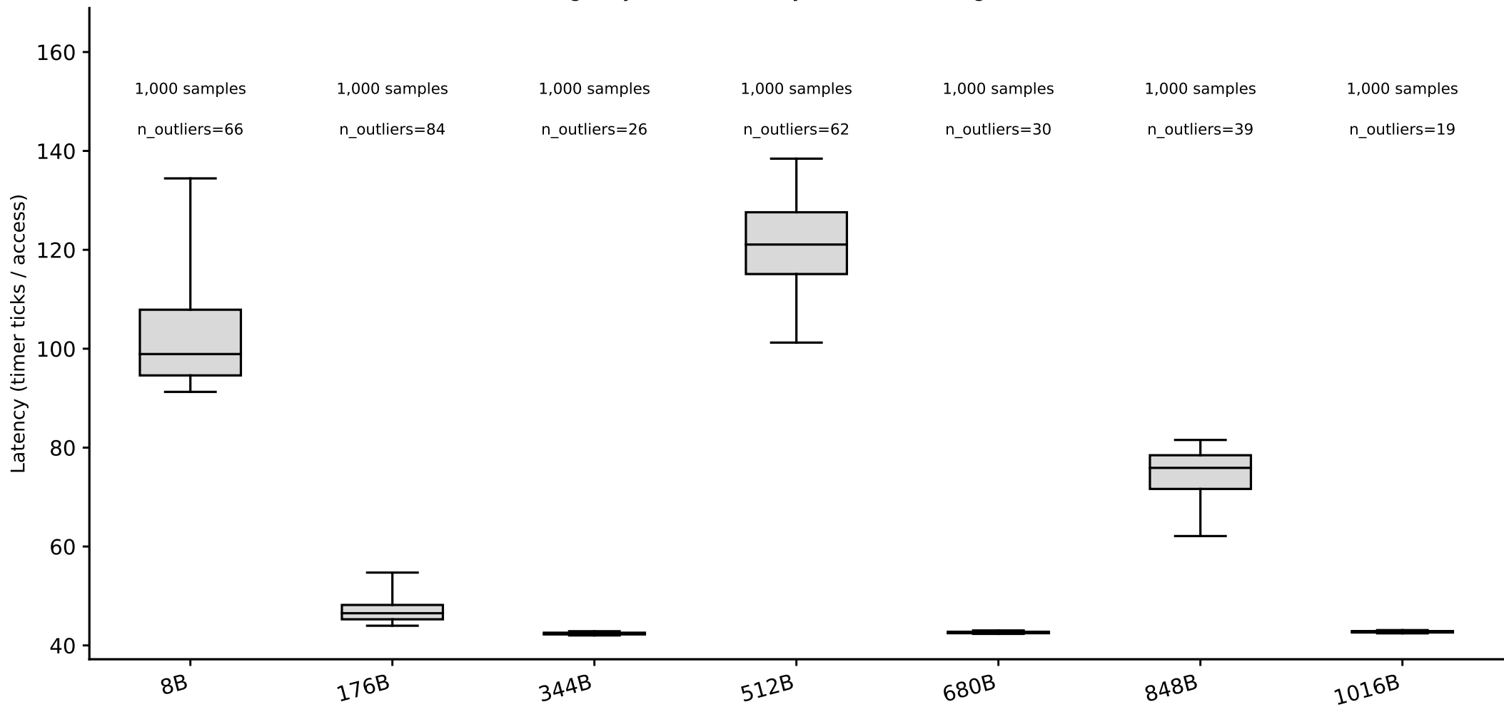
crux: line-size box plots, random pattern (whiskers = p5/p95) (Phase I timing-only, level boundary=8388608B, single-curve method)
