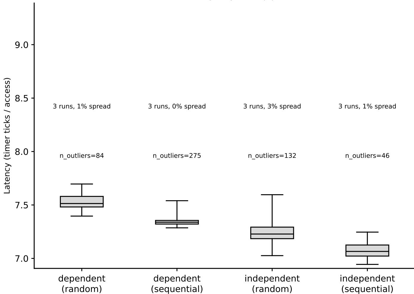
ookay: hit-latency box plots, L1 (footprint=32 KiB) (Phase I timing-only, auto pipeline)
