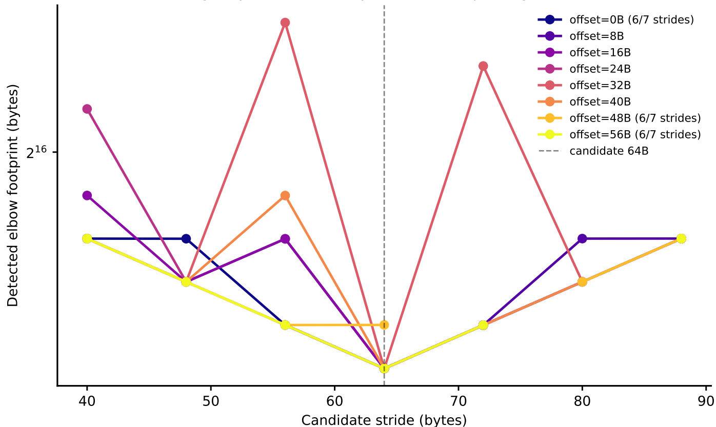
ookay: line-size elbow vs. stride, by node-0 offset (Phase I timing-only, level boundary=32768B, step-4 alignment refinement)
