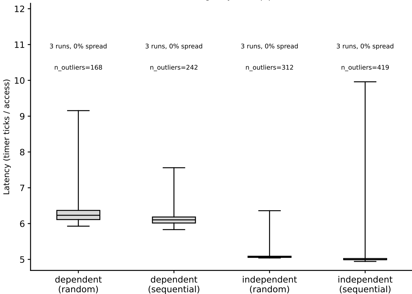
skylark: hit-latency box plots, L1 (footprint=32 KiB) (Phase I timing-only, auto pipeline)
