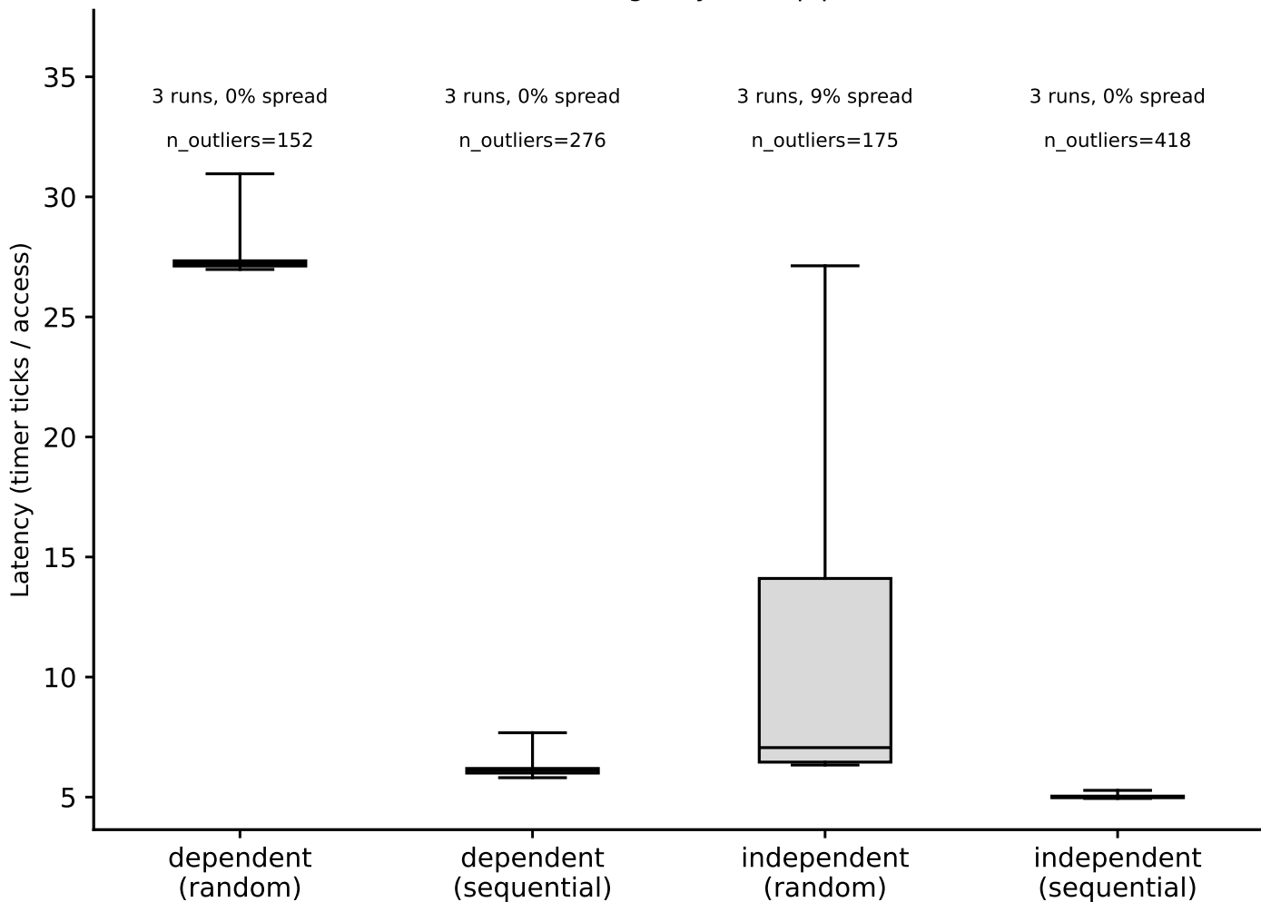
skylark: hit-latency box plots, LLC (footprint=8 MiB) (Phase I timing-only, auto pipeline)
