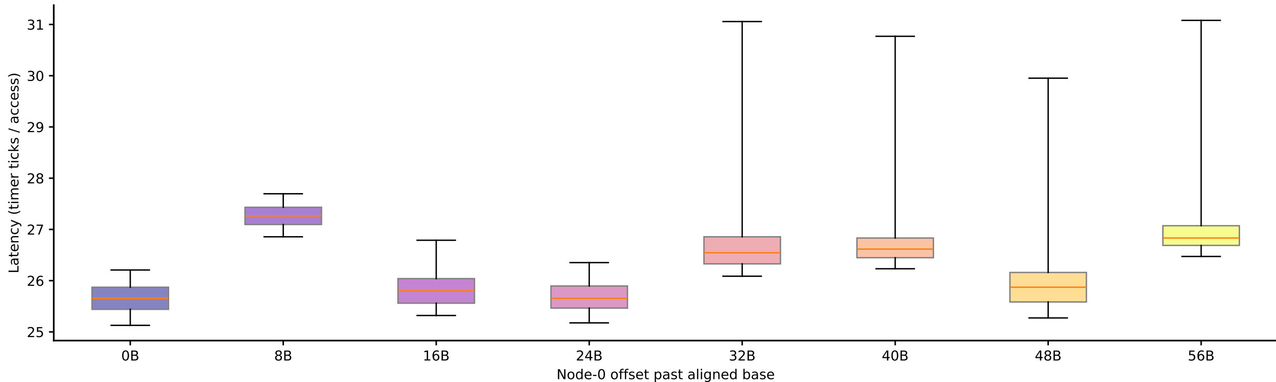
skylark: candidate stride 64 B at footprint 912.25 KiB, by offset (Phase I timing-only, level boundary=524288B, step-4 alignment refinement, candidate=64B)
