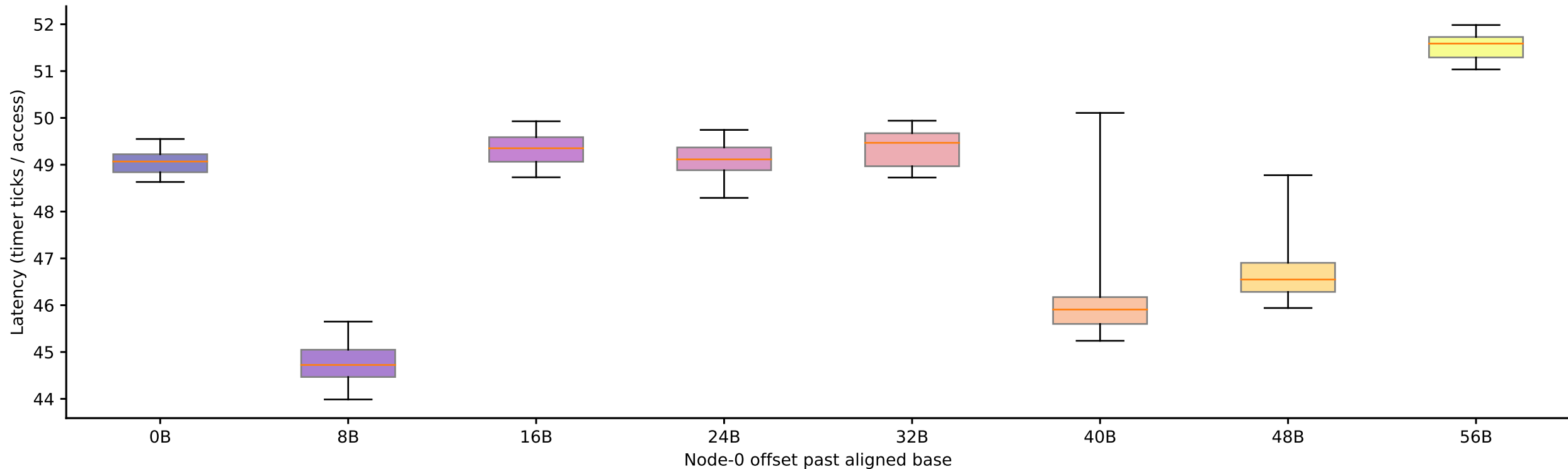
sunbird: candidate stride 64 B at footprint 362 KiB, by offset (Phase I timing-only, level boundary=262144B, step-4 alignment refinement, fresh re-run 20260912T222501Z)
