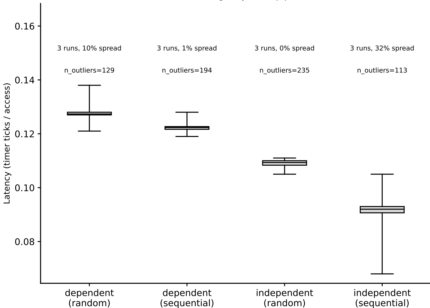
thunderbird: hit-latency box plots, L1 (footprint=64 KiB) (Phase I timing-only, auto pipeline)
