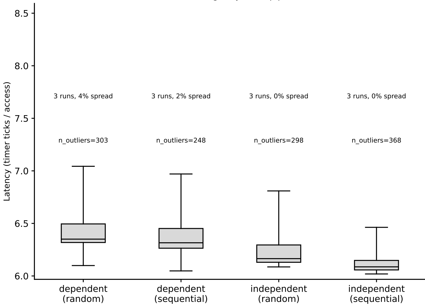
upgrade: hit-latency box plots, L1 (footprint=32 KiB) (Phase I timing-only, auto pipeline)
